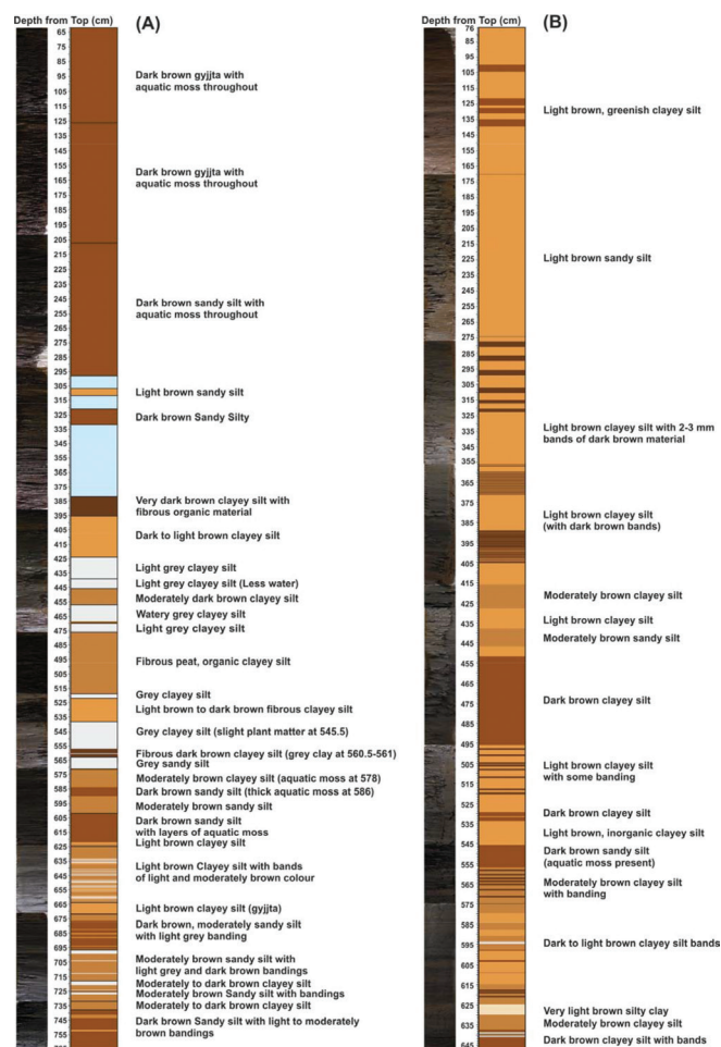
Figure 2: Core photograph with the lithological details. (a) Khajjiar Lake and (b) Rewalsar Lake.
