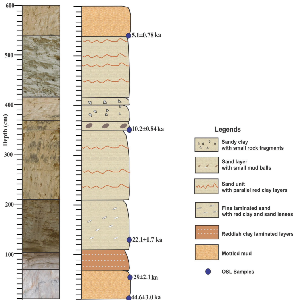
Figure 2: Litholog of Bhikiyasain palaeolake profile.
